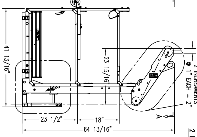
WORK BASKETS PASS THROUGH DIMENSIONS
