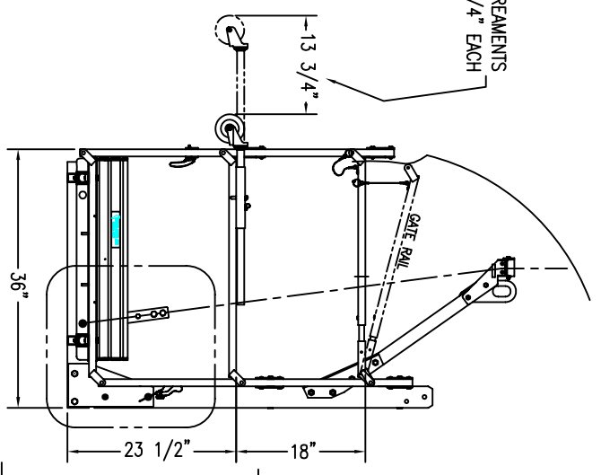
WORK BASKETS PASS THROUGH DIMENSIONS
