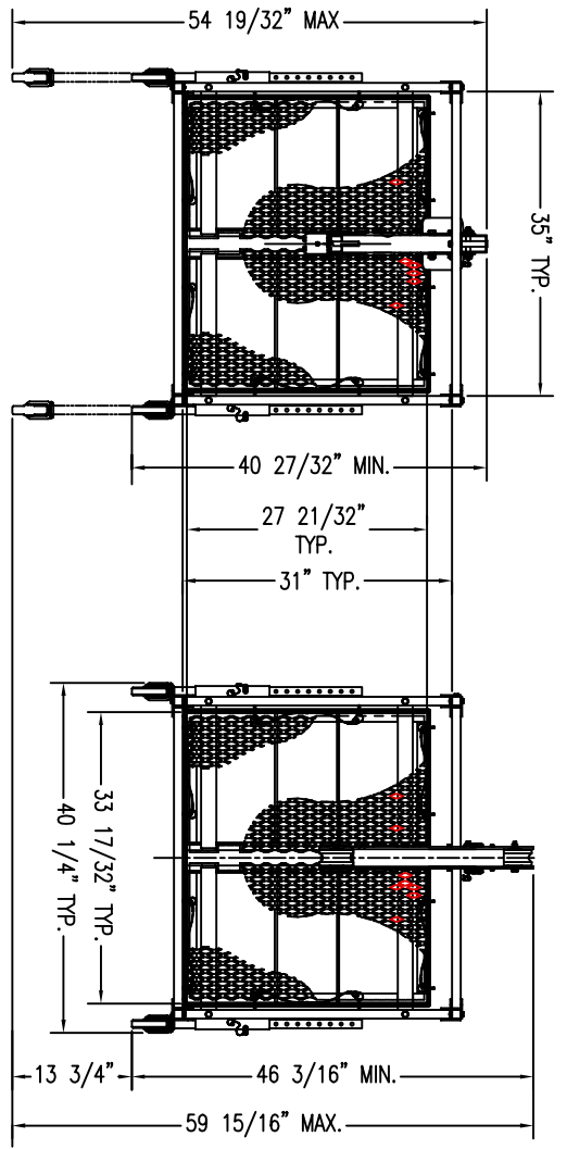
EXTERIOR MOUNT SECTION A-A
